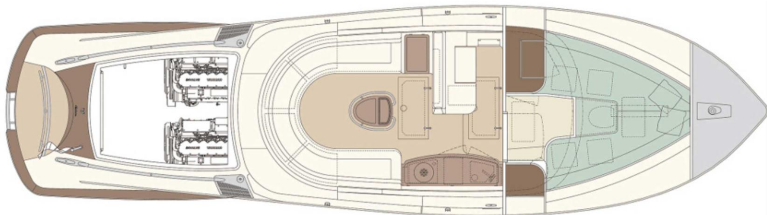
Main deck
